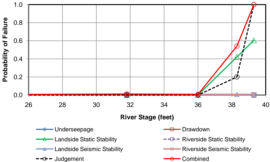
Skagit River Levee General Investigation Levee Risk and Reliability Analysis Skagit County, Washington FRAGILITY CURVE AND TABLE SECTION DD17-2L January 2011 21-1-21199-003 SHANNON & WILSON, INC. Geotechnical and Environmental Consultants FIG. 27
