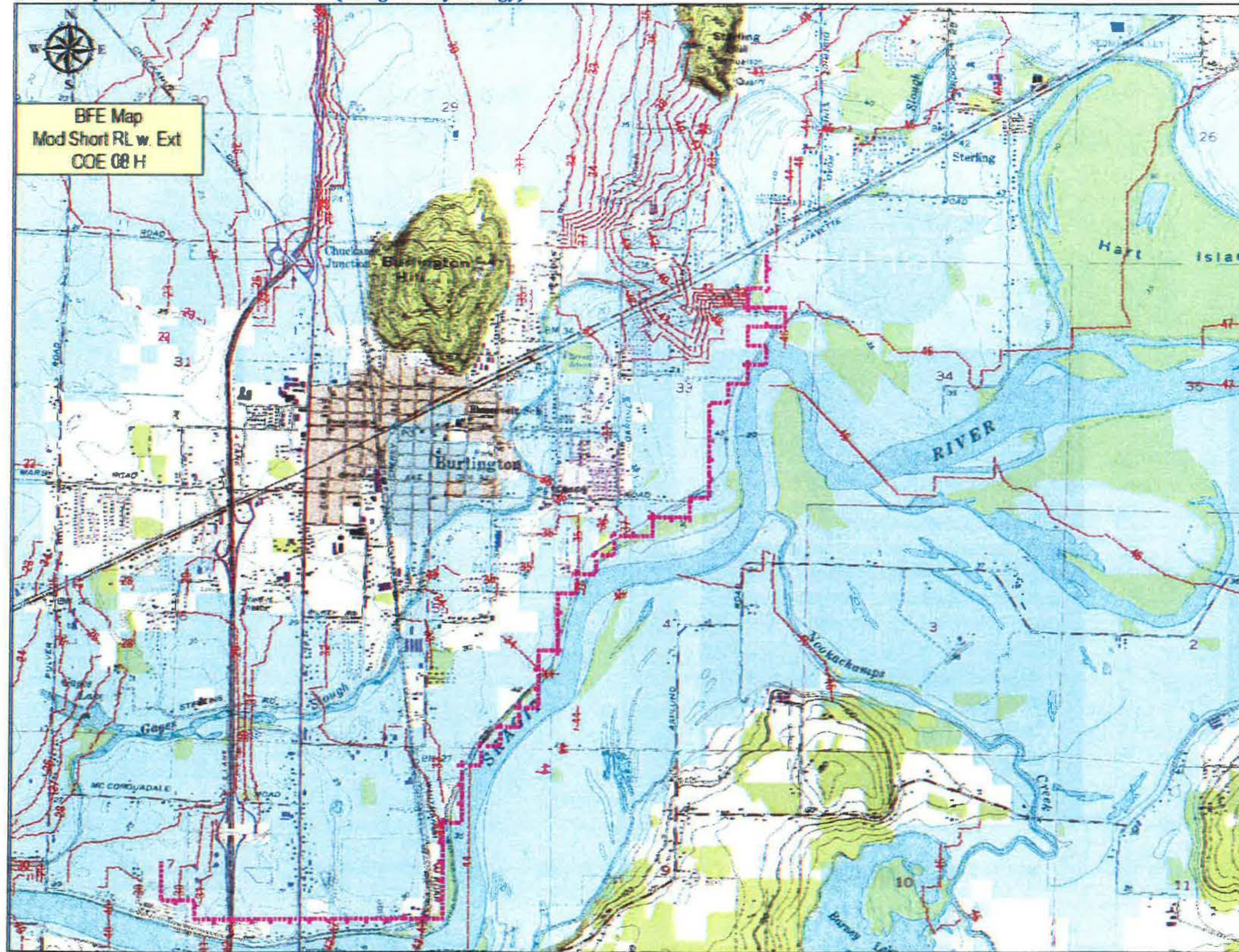
BFE Map - Proposed Certified Levee (using COE Hydrology)
