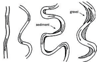
The evolution of a meandering channel.
