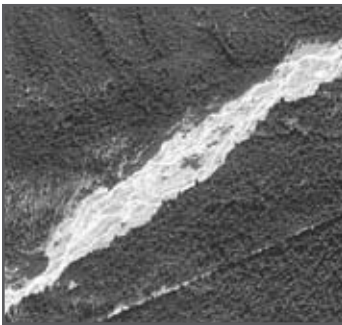
Aerial view of a braided channel.
