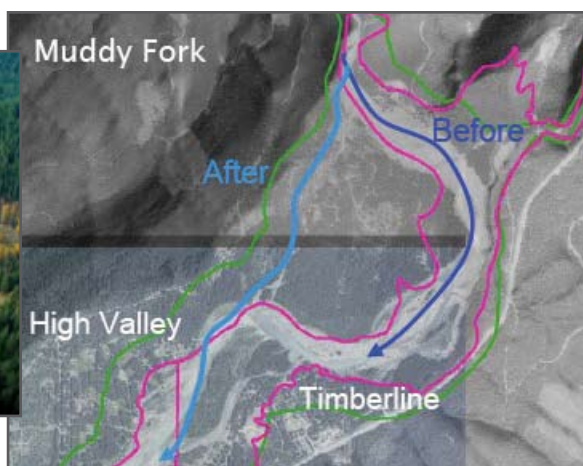
Aerial views of the Muddy Fork–Cowlitz River confluence.
